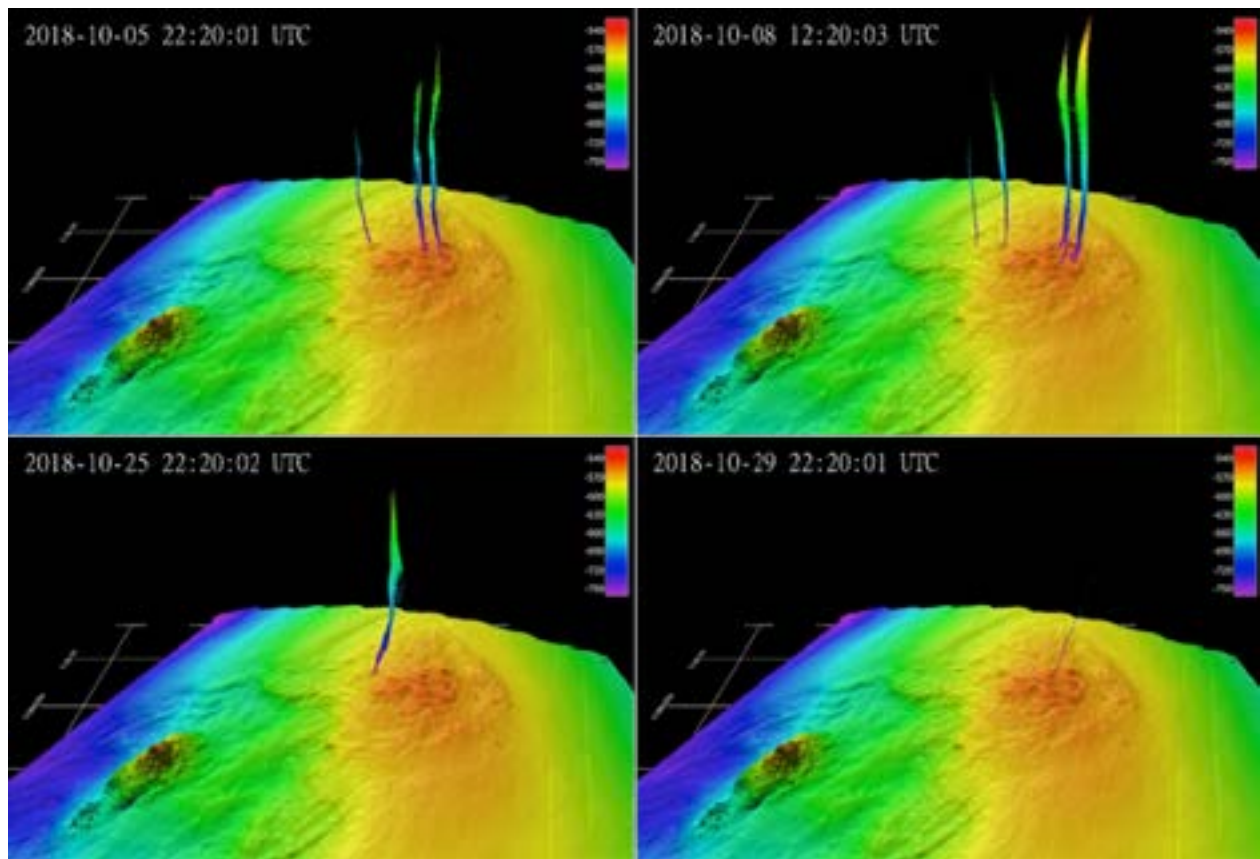
FIGURE 2.14 Methane bubble emissions detected by the MARUM overview sonar over the Southern Hydrate Ridge summit. The location and size of the bubble plumes vary considerably over time.
