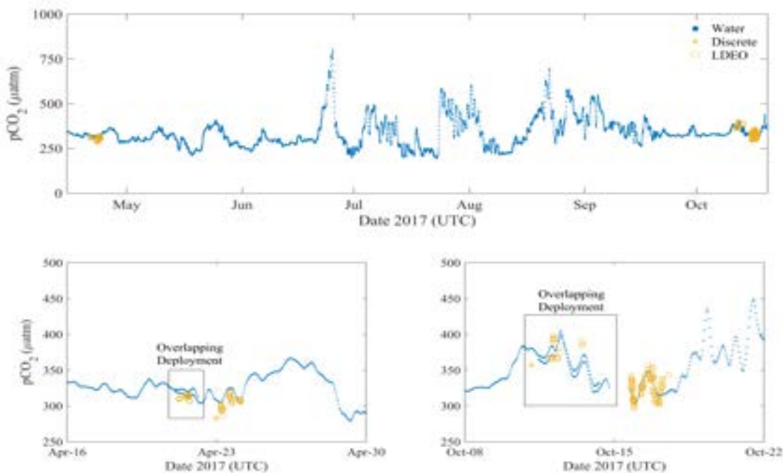
FIGURE 2.7 Surface water pCO 2 for the Spring 2017 deployment of the Endurance Oregon shelf mooring (Wingard et al., 2020). Note the high degree of variability during the summer, which is similar to other observations made on the Oregon Shelf (Evans et al., 2011). This plot also shows the observed offsets between the surface water pCO 2 measurements (blue dots, •) and the discrete bottle samples (yellow asterisks, *) and the LDEO Underway Database (yellow open circles). Detailed views in the lower two panels show the offsets during the periods of over-lapping deployments. The independent measurements obtained by the separate systems, and the close agreement between them, provide measures of confidence in the accuracy and applicability of the data.
