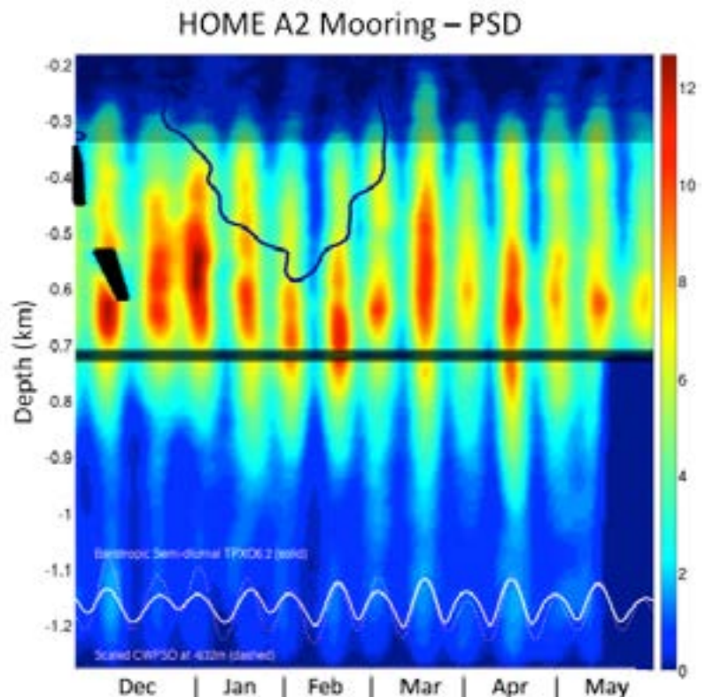
FIGURE 2.4 The horizontal velocity power spectral density (PSD; m^2/(\text{rad/s}) ) of semidiurnal ITs over a six-month time period, as a function of depth. Data are from a mooring at Kaena Ridge in Hawaii collected during 2002 (Carter et al., 2008).
