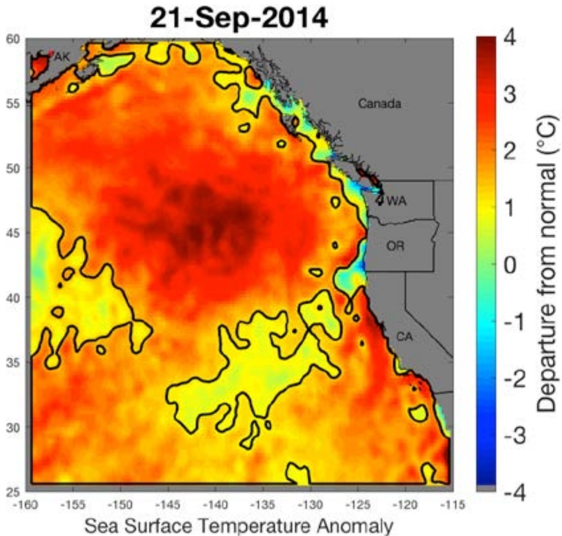
FIGURE 2.3 The 2013-2015 Northeast Pacific marine heatwave known as “The Blob” on the date when it reached its maximum size. Color represents sea surface temperature anomaly from NOAA’s OISST dataset ( https://www.ncdc.noaa.gov/oisst ), dark contour denotes the region which classifies as a “heatwave” by the definition of Hobday, 2016.
