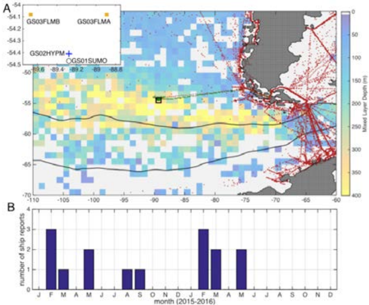
FIGURE 2.5 (a) Map of region near the Ocean Observatories Initiative (OOI) mooring array (black rectangle) with the climatological monthly mean August mixed layer depth; (b) total number of ship-based meteorological reports in the ICOADS3.0 data set with sufficient data to estimate latent heat flux obtained within 500 km of the OOI mooring site for each month of 2015 and 2016, excluding all OOI mooring deployment and recovery cruises. From Ogle et al., 2018
