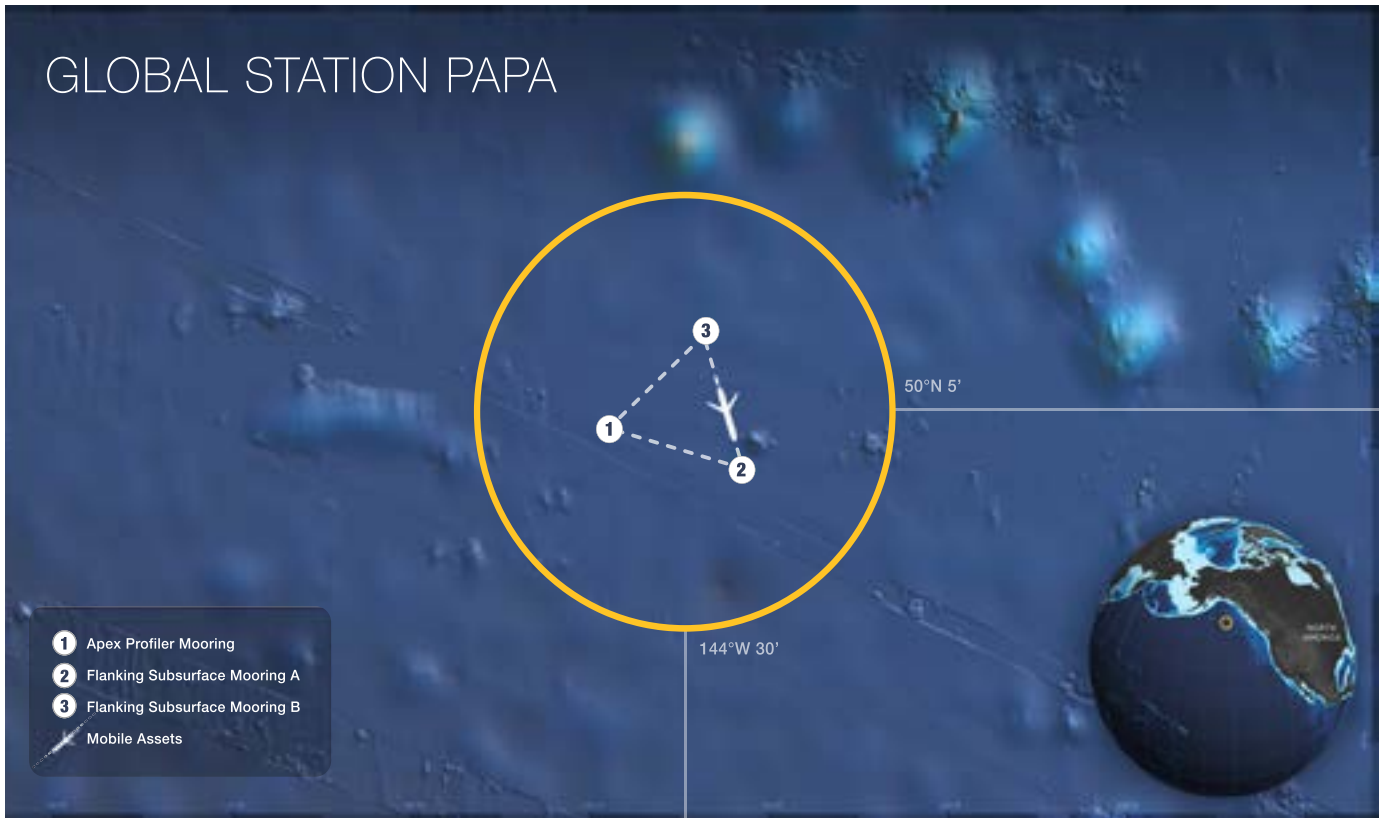
FIGURE 3.2 Located in the Gulf of Alaska, Global Station Papa is in a region with a productive fishery, low eddy variability, and vulnerable to ocean acidification. Credit: Center for Environmental Visualization, University of Washington
