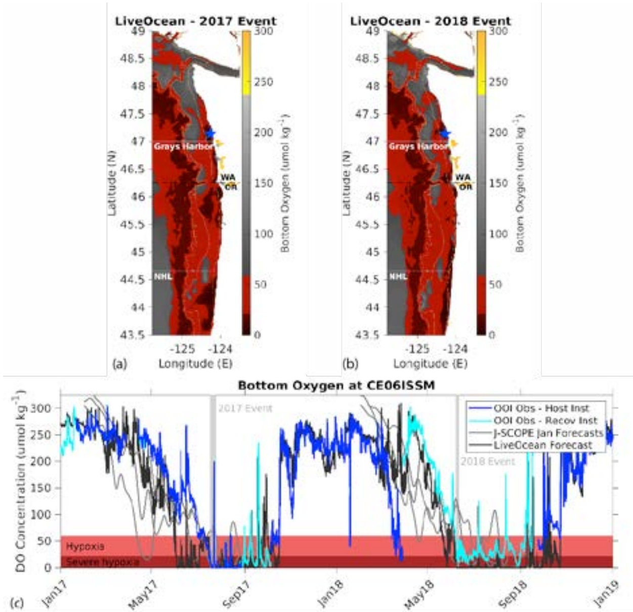
FIGURE 2.8 Forecasted and observed hypoxia along the Washington and Oregon coasts in 2017 and 2018 as depicted by the dissolved oxygen concentration (DO) along the bottom. Maps of the LiveOcean forecasted bottom oxygen fields for the (a) 2017 and (b) 2018 events respectively. The time series of 2017–2018 is provided in (c) from the moored observations from the “host” and “recovered” data streams at the Washington Inshore Surface Mooring of the OOI’s Regional Endurance Array (CE06ISSM, blue line, blue star on (a) and (b)). Forecasts are also provided in (c) over the same time period for the same location from LiveOcean (black) and J-SCOPE (grey, three ensemble members, January-initialized). Hypoxic and severe hypoxic conditions are highlighted in all panels by red and dark red respectively. Figure assembled by Emily Norton.
