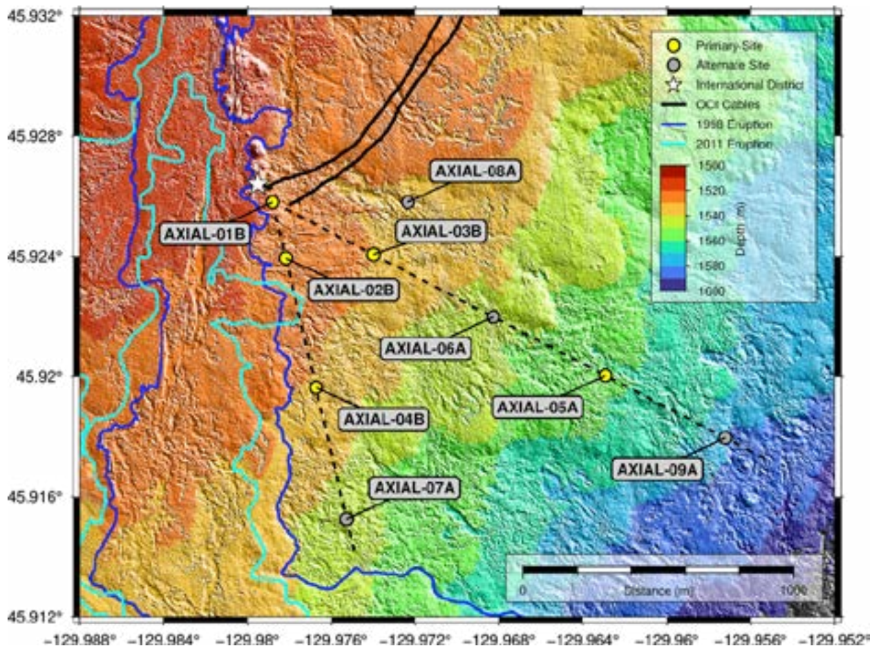
FIGURE 2.13 Bathymetric map with proposed drill sites as part of IODP 955-Full. Site AXIAL-01B is situated approximately 50 m southwest of International District, and between RCA cable junction boxes MJ03C and MJ03D.
