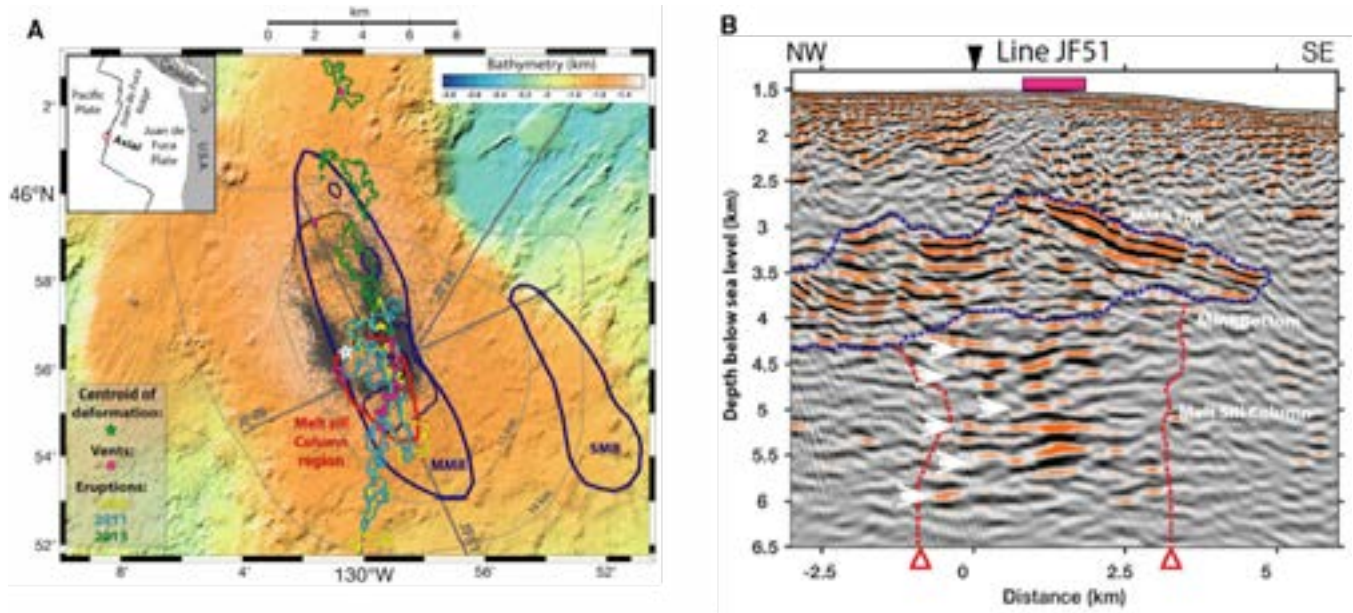
FIGURE 2.12 A. Bathymetric map showing location of mid-lower crust melt-mush conduit (red line) and relationships with other magmatic features including upper-crustal Main and Secondary Magma Reservoir (MMR and SMR) identified in Arnulf et al [2014; 2018] in blue with shallowest portion (2.9 km bsl) in thinner line. Recent lava flows are color coded for eruption year as in legend and hydrothermal vent fields indicated with purple dots. Green star marks centroid of pressure source from Nooner and Chadwick [2016] and white star is revised location from Hefner et al., [2020]. Black dots show seismicity detected prior and during the 2015 eruption [Arnulf et al., 2018]. B. Reverse Time Migration image showing melt lens conduit beneath MMR at Axial, along lines 51. Blue line indicates interpreted top and bottom of MMR. Red lines delineate melt column region. Figure modified from Carbotte et al. [2020].
