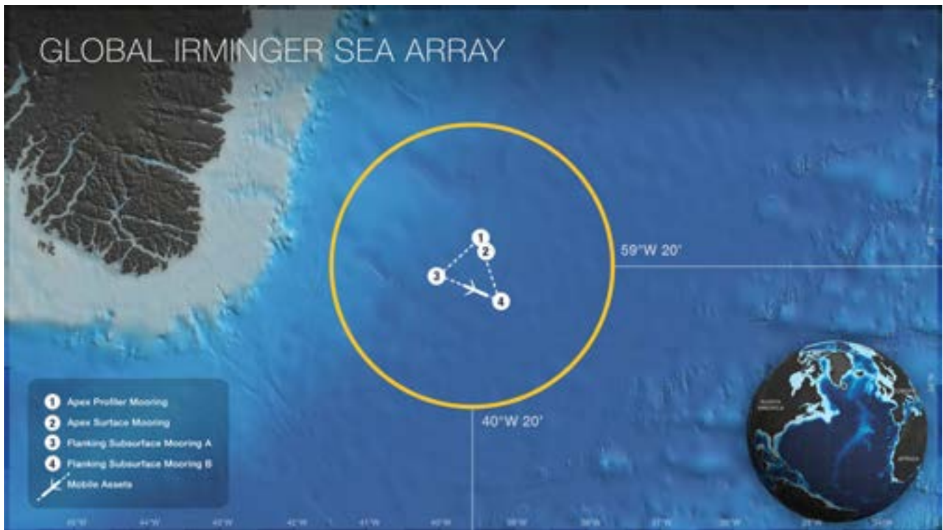
FIGURE 3.4 The Irminger Sea Array was selected as one of OOI's array sites because it is one of the few places on Earth with deep-water formation that feeds the large-scale thermohaline circulation.. Credit: Center for Environmental Visualization, University of Washington
