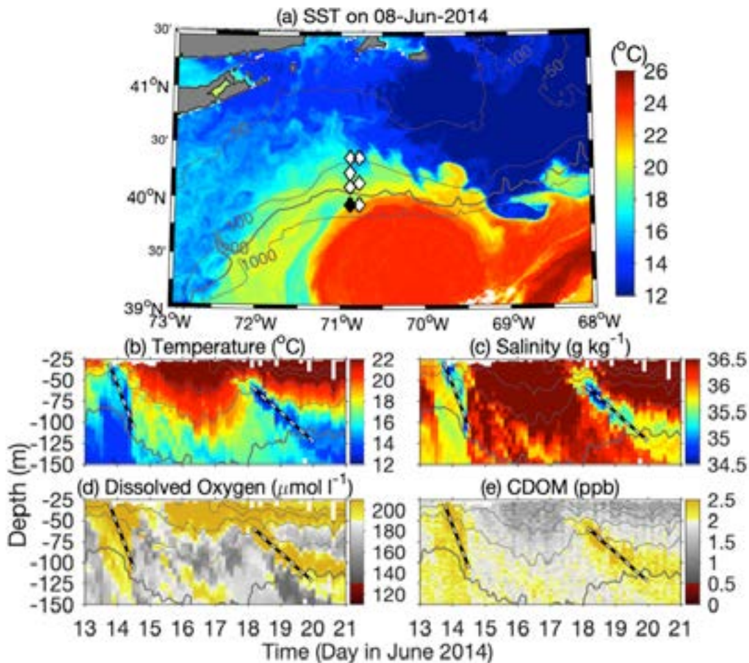
FIGURE 2.9 (a) Sea surface temperature on June 8, 2014, showing a warm core ring impinging on the shelfbreak near the Pioneer Array moorings (diamonds). Time series of (b) temperature, (c) salinity, (d) DO, and (e) CDOM from the Offshore mooring (black in (a)). Grey contours in (b–e) are isopycnals, with a contour interval of 0.25 kg m -3 and the 26.5 kg m -3 isopycnal bold.
