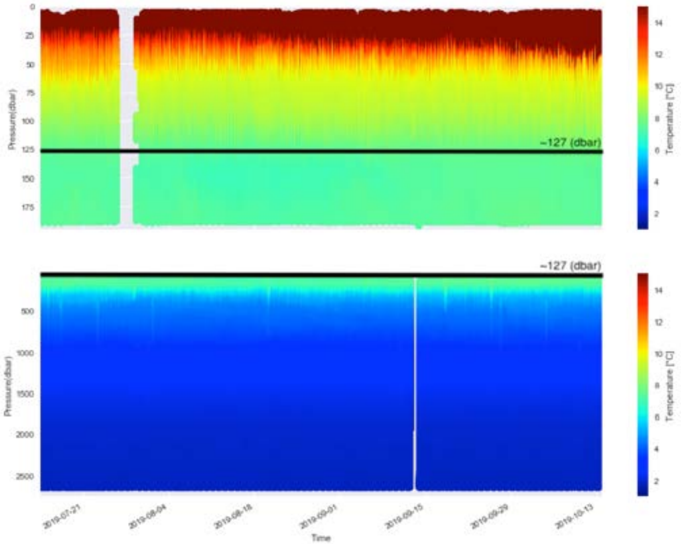
FIGURE 7.3 Visualization of temperature across the same time range for different depth ranges. Shallow Water Profilers profile from ~5 m to 200 m below the sea surface; Deep Water Profilers profile from ~150 m to 2900 m below the sea surface. These two sensor platforms can be used to investigate parameters throughout the full water column depth.
