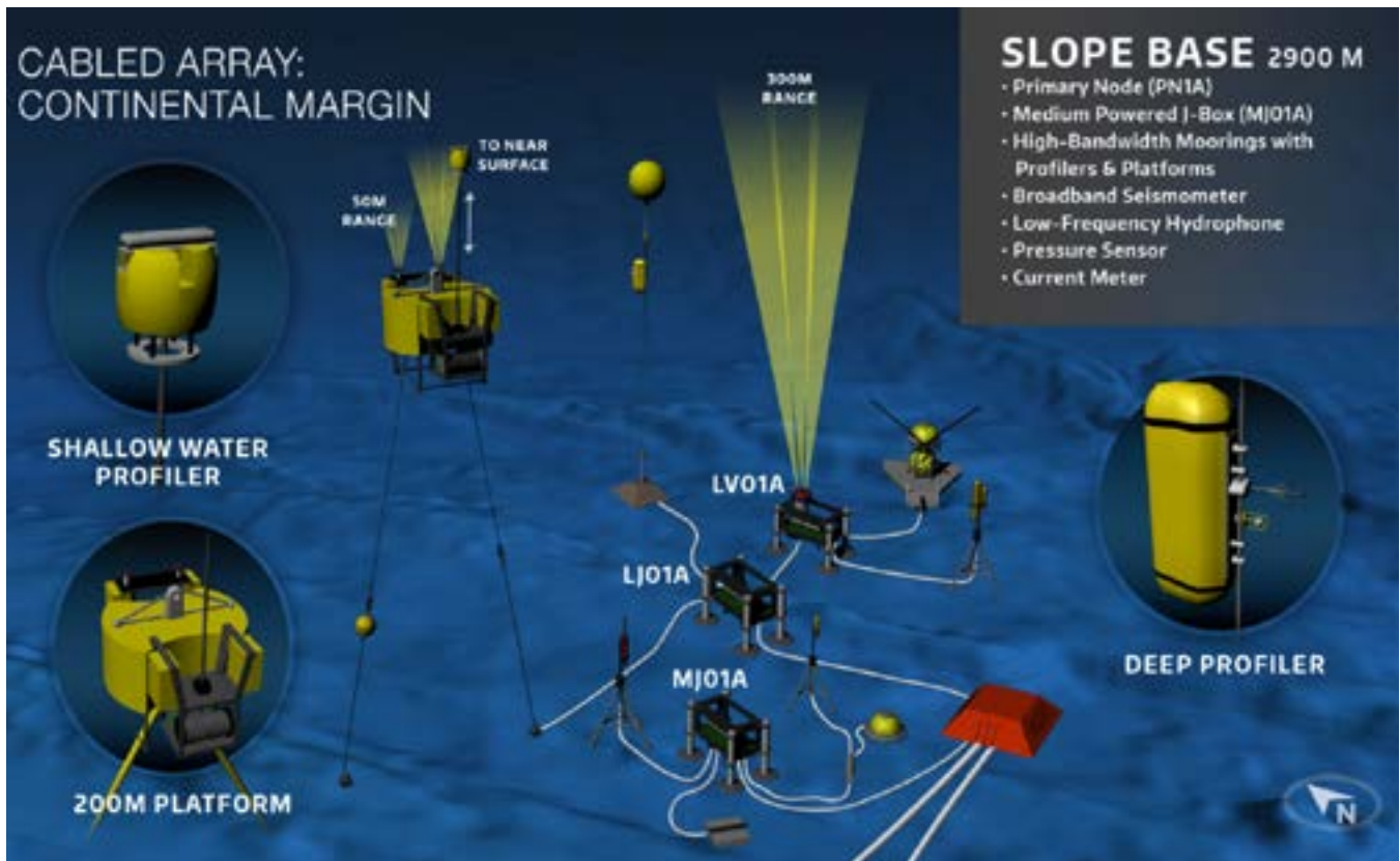
FIGURE 3.13 Slope Base: Junction Boxes host geophysical instruments and others focused on water column processes. These are paired with a Cabled Deep Profiler Mooring and a Cabled Shallow Profiler Mooring. Credit: Center for Environmental Visualization, University of Washington
