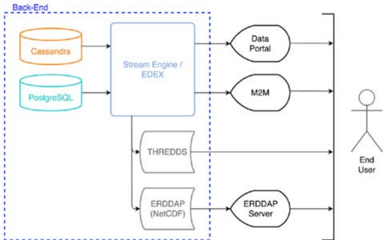
FIGURE 3.20 Simplified diagram showing the relationship of OOI CI back-end components and three of the user-facing data service systems.
