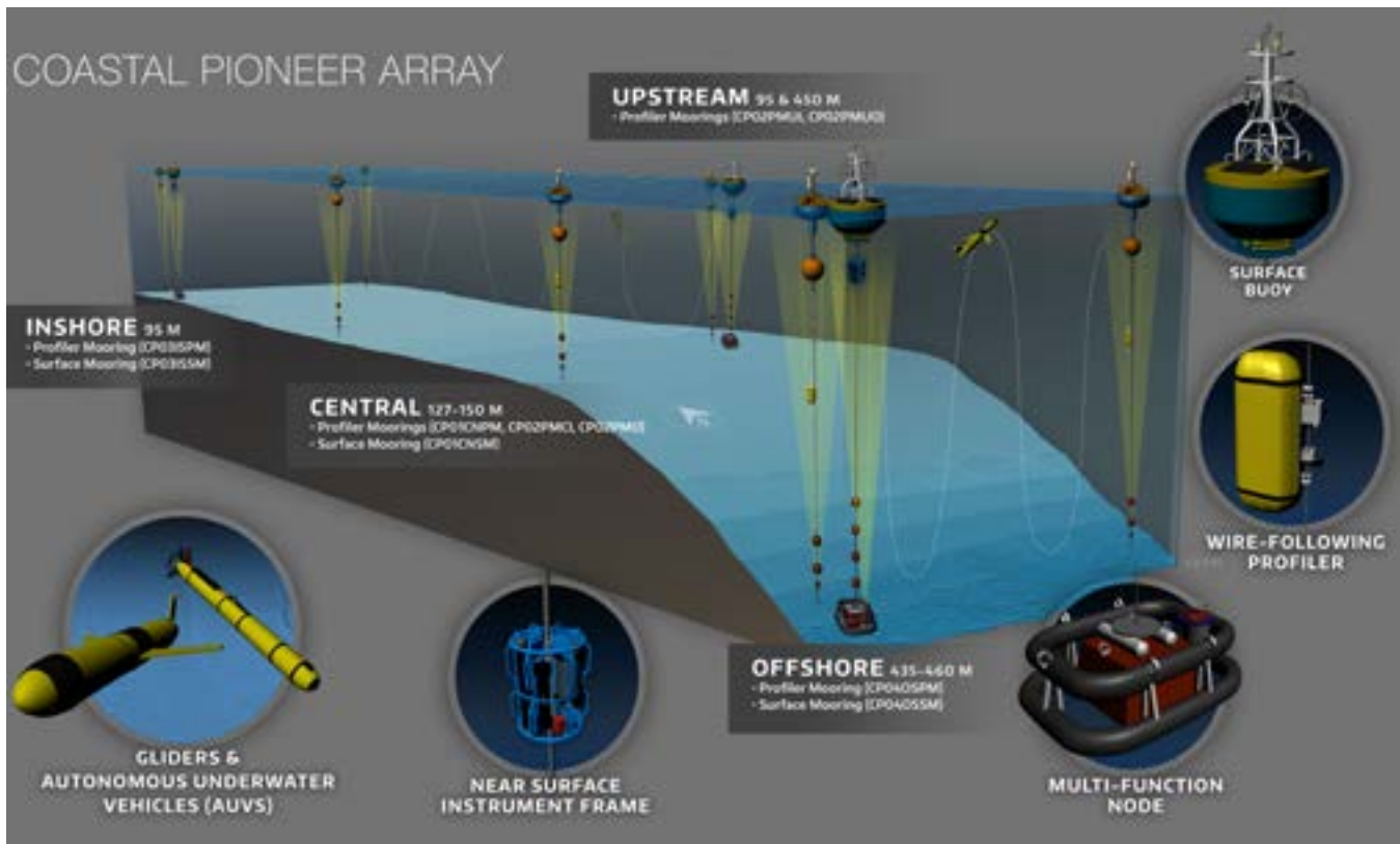
FIGURE 3.19 Pioneer’s mooring array utilizes two different mooring types-- Surface Moorings and Profiler Moorings. contain wire following profilers and upward-looking Acoustic Doppler Current Profilers. Moorings are supplemented by coastal gliders , profiling gliders, and autonomous underwater vehicles (AUVs). Credit: Center for Environmental Visualization, University of Washington
