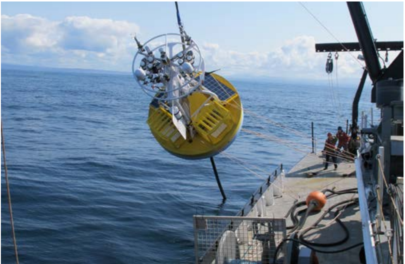
FIGURE B. The Oregon shelf surface mooring is lowered to the water using the R/V Oceanus ship's crane. Credit: OOI Endurance Array Program, OSU.
