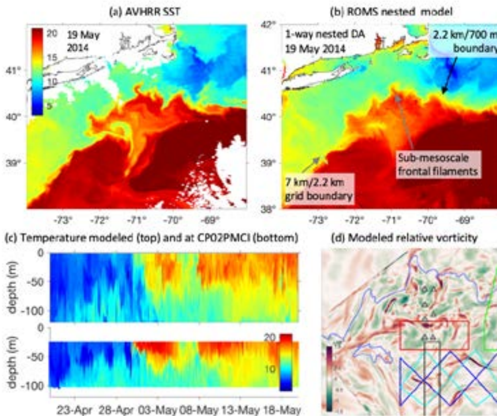
FIGURE 2.11 Surface temperature and relative vorticity during an across-shelf intrusion event studied by Zhang and Gawarkiewicz (2015).
