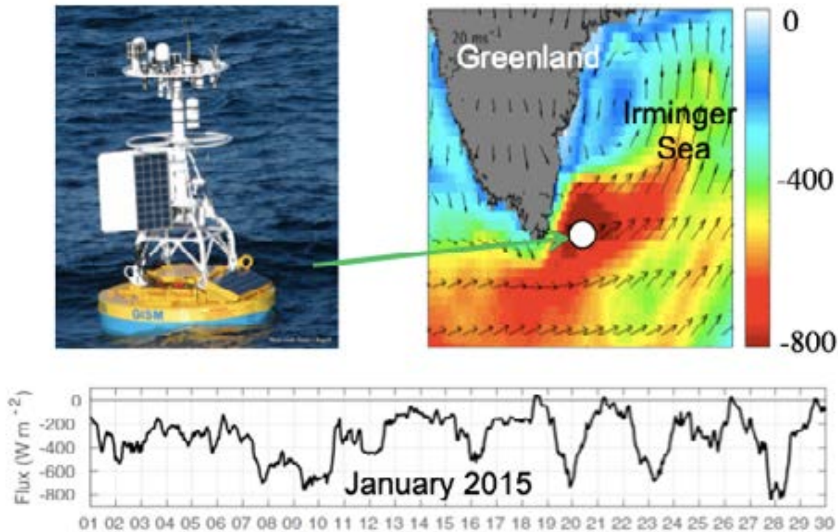
FIGURE 2.6 Top left – The OOI Irminger Surface Mooring. Top right – Mooring deployment location (white circle) together with ERA5 reanalysis ocean heat loss (colour, \text{Wm}^{-2} ) and winds (arrows). Bottom – Time series of the hourly mean net air-sea heat flux in an example month (January 2015) with intense Greenland Tip Jet related ocean heat loss up to 800 \text{ Wm}^{-2} .
